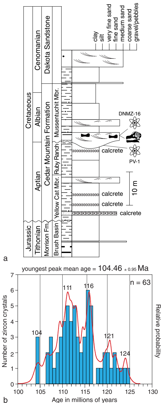
Fig. 2 Stratigraphy and geochronology of DNM 16. a Stratigraphic section indicating position of skulls and zircon samples DMMZ-16 and PV-1. b Histogram of number of zircon crystals ( blue ) and relative age probability curve ( red ) of single crystal detrital zircon U/Pb dating of sample PV-1, the mudstone underlying the bone-bearing sandstone; 104.46 \pm 0.95 Ma = Youngest Peak Mean Age, 2 sigma (3 crystals, mean square weighted deviation = 0.0112, probability = 0.099). See Online Resources 1 and 2 for geochronologic data
