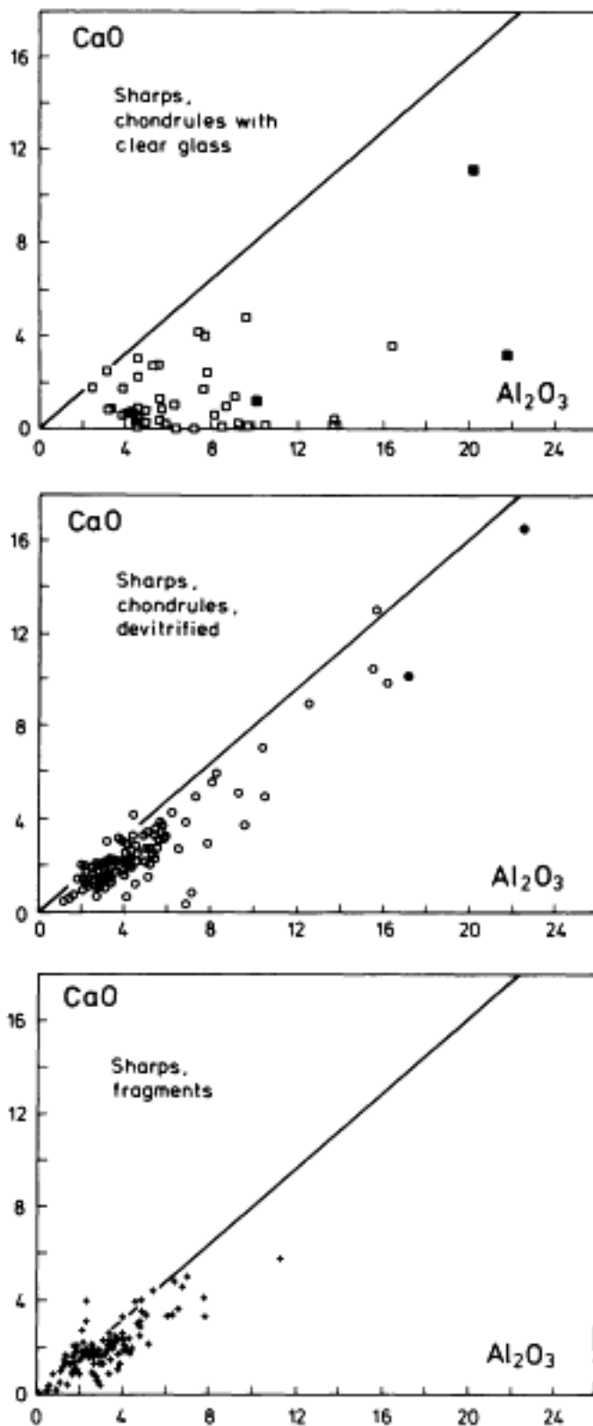
Fig. 9 CaO vs. \text{Al}_2\text{O}_3 (wt.%) for bulk chondrules and fragments from Sharps. The straight line gives the chondritic Ca/Al ratio (Ahrens et al. , 1969). Filled symbols are for Ca,Al-rich chondrules with Ti-augite and spinel.
