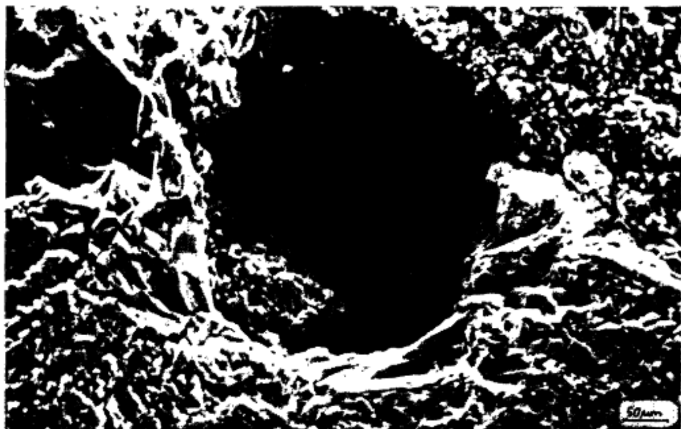
Fig. 6 Large vesicle in chondrule in Fig. 5, enlarged.
