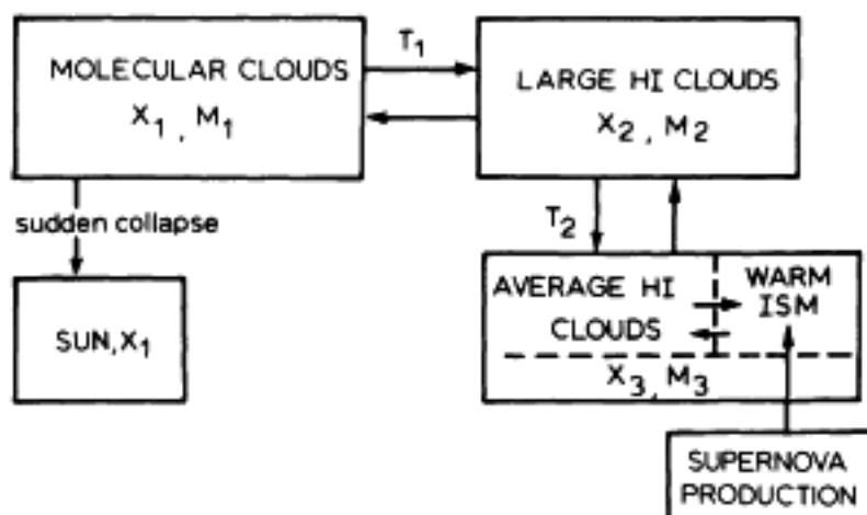
Fig. 2 Schematic diagram for the transport of fresh radioactivities made in supernova explosions into the collapsing solar system. The concentration X_1 in molecular clouds is determined by mass exchange with surrounding large HI clouds on a time scale T_1 . The concentration X_2 in the large HI clouds is governed by the time scale T_2 with which they exchange matter with average HI clouds. Because supernova shocks evaporate average HI clouds, their mass is included with that of the hot media in the initial reservoir for fresh radioactivities.
