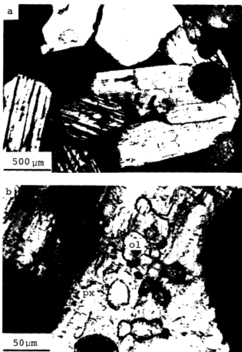
Fig. 7 (a) Experimentally reproduced porphyritic pyroxene texture with poikilitically enclosed olivine. The charge was heated at temperature 15°C below the liquidus temperature for 2 minutes and cooled at a rate of 5°C/hr. (b) Poikilitically enclosed olivine in pyroxene shown in Fig. 6. Ol=olivine. Px=pyroxene.
