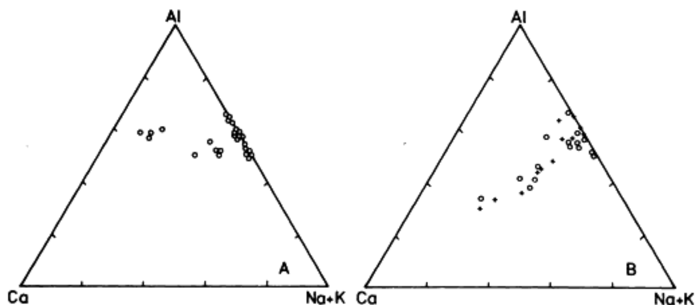
Fig. 11 Three-component plot for mesostases from Sharps (in wt.% of oxides). (a) clear glass; (b) devitrified glass in chondrules (o) and fragments (+).
