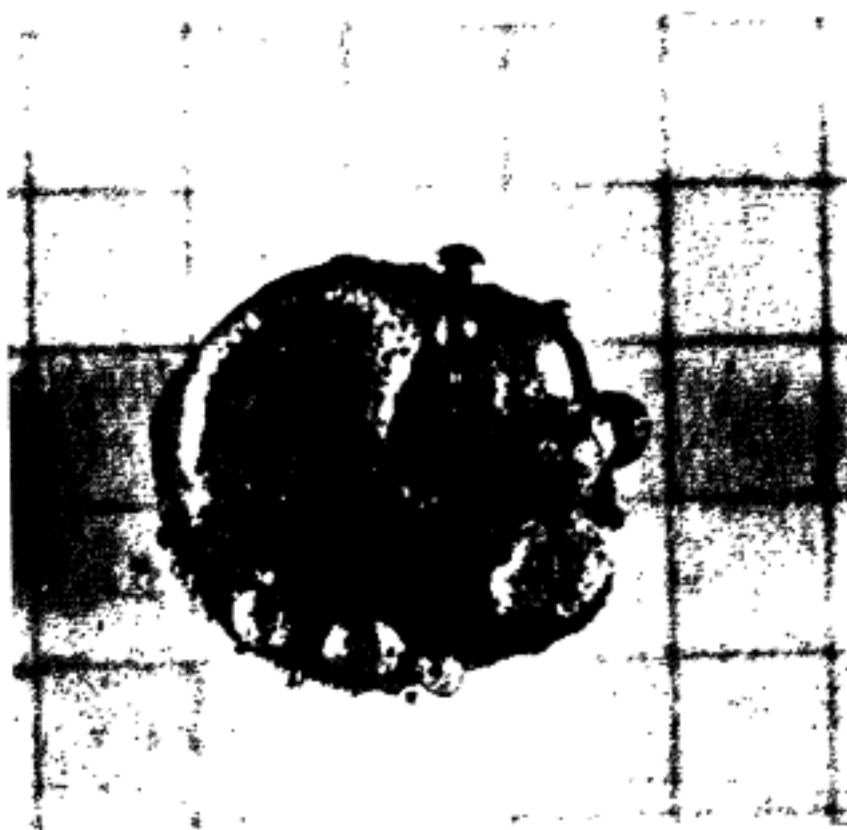
Fig. 2 Bottom of the residual melt bead formed from the fusion and partial evaporation in the solar furnace in vacuum ( <1 mm Hg) of powdered bulk Allende showing numerous large iron spherules on the periphery of the bead. Spacing of the background grid is approximately 2.5 mm between adjacent parallel lines.
