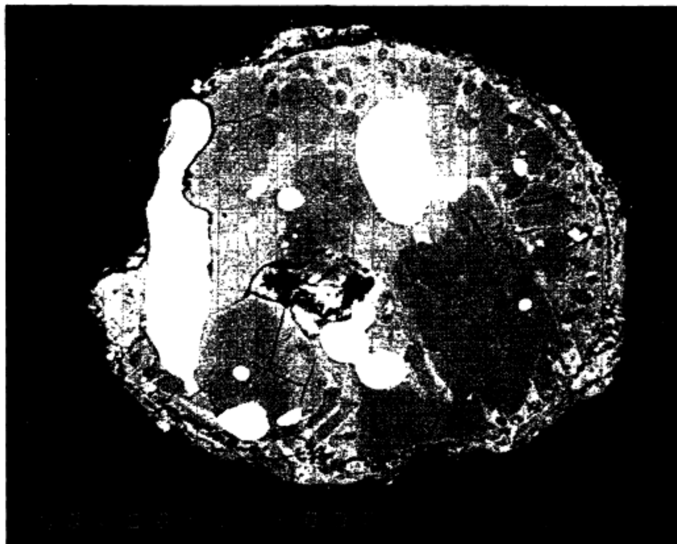
Fig. 1 Chondrule 3A, 280 micrometers in diameter. Silica pods are the darkest shade of gray. Pale gray patches are residual glasses (col. 5 in Table 2). Medium gray shades are enstatite. Small, whitish-gray grains are calcic-pyroxene. Bright white is metal. (During section preparation a grain was plucked out of the approximate center of the chondrule, leaving a hole.)
