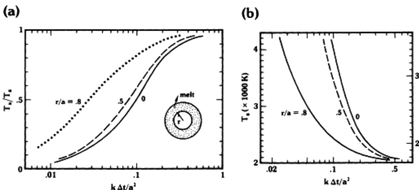
Fig. 1 (a) Normalized maximum attainable temperature ( T_x/T_s ) vs. the heating duration ( k \Delta t/a^2 ) at radial distances ( r/a ) of 0.8, 0.5, and 0 for an externally heated chondrule. (b) The surface temperature ( T_s ) vs. the heating duration of T_s for liquidus of 2000 K (left-hand scale) and of 1700 K (right-hand scale).
