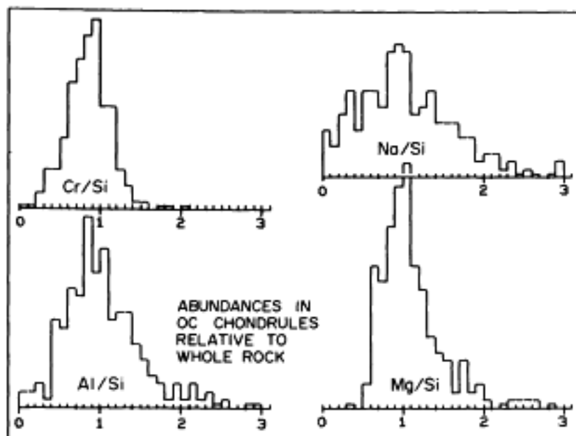
Fig. 5 Histograms of ordinary chondrite chondrule compositions. These data are normalized to mean ordinary chondrite values: \text{Al/Si} = 0.081 , \text{Mg/Si} = 0.88 , \text{Cr/Si} = 0.12 , and \text{Na/Si} = 0.043 g/g. Four hundred individual chondrule analyses were used, 100 of which had no Cr determination. The widest ranges occur for Al and Na, with volatility far from that of Si, the normalizing element; the smallest ranges are seen in Cr and Mg, which are similar in volatility to Si.
