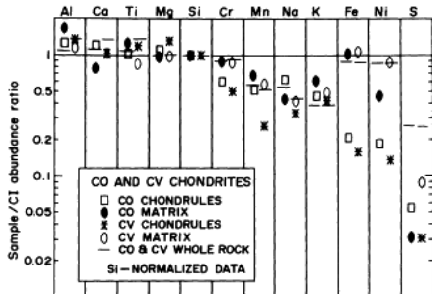
Fig. 4 The grand mean compositions of CO chondrules and CV chondrules (McSween, 1977a,b; Simon and Haggerty, 1980) are plotted together with the compositions of coexisting fine-grained matrix (McSween and Richardson, 1977) and whole-rock CO and CV chondrites. The data are normalized to CI chondrites and to Si. Chondrule lithophile/Si ratios are similar to those in whole rock except for Mg/Si, which is higher, and Cr/Si and Mn/Si, which are lower than in whole rock. Matrices show variations similar to those in ordinary chondrites.
