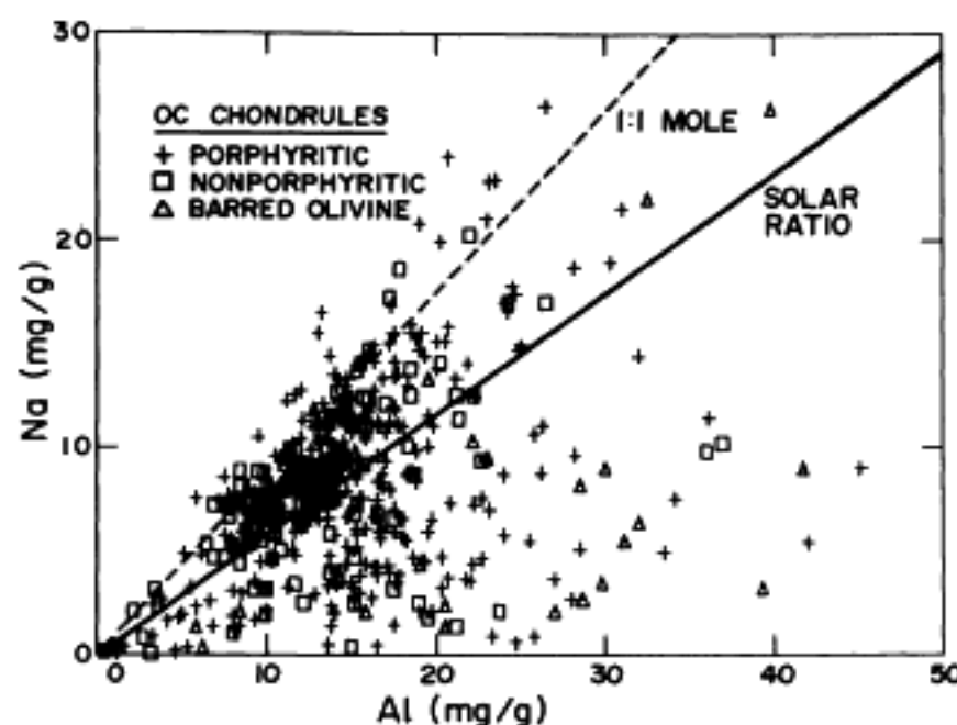
Fig. 14 Sodium vs. Al concentrations in unequilibrated OC chondrules. The solar ratio is shown as a solid line, and the 1:1 mol. ratio is shown as a dotted line. The mean chondrule composition is near the solar ratio; relatively few chondrules have Na/Al ratios above the 1:1 line, even at low Al contents. Recondensation of Na onto chondrule surfaces probably did not occur. The Na/Al ratio is probably controlled by condensation processes involving the precursor solids.
