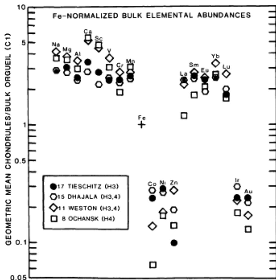
Fig. 1 "Average" elemental abundances in whole chondrules separated from mildly to highly unequilibrated H-group chondrites. This plot was constructed by normalizing geometric-mean data sets in Table 2 (and Table 1 of Gooding et al. , 1980a) to total Fe concentration and then, for each element, dividing the result by the Fe-normalized abundance in the bulk Orgueil (C1) chondrite as derived from the geometric-mean data reported for Orgueil in Table 2 of Gooding et al. (1980a). Elements are listed, from left to right, in order of increasing atomic number.
