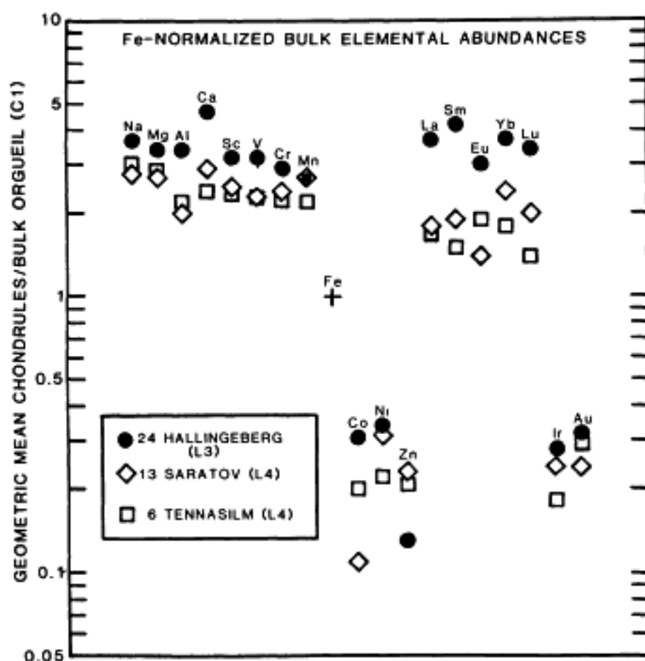
Fig. 2 "Average" elemental abundances in whole chondrules separated from mildly to highly unequilibrated L-group chondrites. Details are the same as given for Fig. 1.
