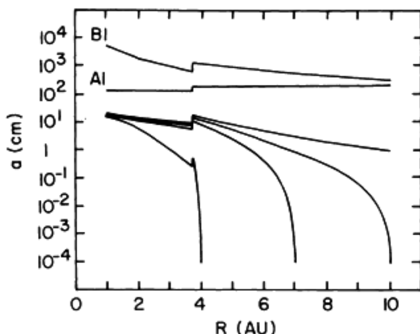
Fig. 2 Size of the test particle vs. radius using Weidenschilling's model. The background-particle size and the sticking probability are 1 \mu\text{m} and 0.1, respectively. The test particle starts out with 1 \mu\text{m} in size at 4, 7, and 10 AU and with 1 cm at 10 AU. The radial motion is approximated by the drift owing to gas drag. Curves A1 and B1 show how large particles must be to either: (A1) begin minimizing radial drift resulting from gas drag; or (B1) to decouple from the turbulence.
