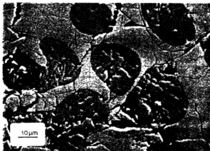
Fig. 3 Backscatter electron micrograph showing cristobalite(?) dendrites and interdendrite voids within silica ellipsoids (dark grey) and the unperturbed interface between spherulitic iron magnesium silicate matrix (medium grey) and silica.
