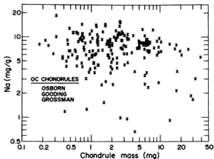
Fig. 6, a plot of Na concentration vs. chondrule mass, and Fig. 7, Na/Al vs. mass. Dilution effects of metal/sulfide were neglected. As in the work on thin sections, the predicted correlations are not observed.
