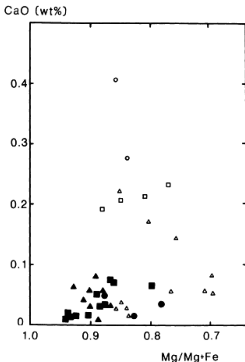
Fig. 5 Relationship between Mg/Mg + Fe ratios and CaO content of poikilitically enclosed olivine in three chondrules in ALH-77015 chondrite. Closed symbols: olivine larger than 100 \mu\text{m} . Open symbols: olivine smaller than 20 \mu\text{m} . Solid and open marks of same symbols are in a single chondrule.
