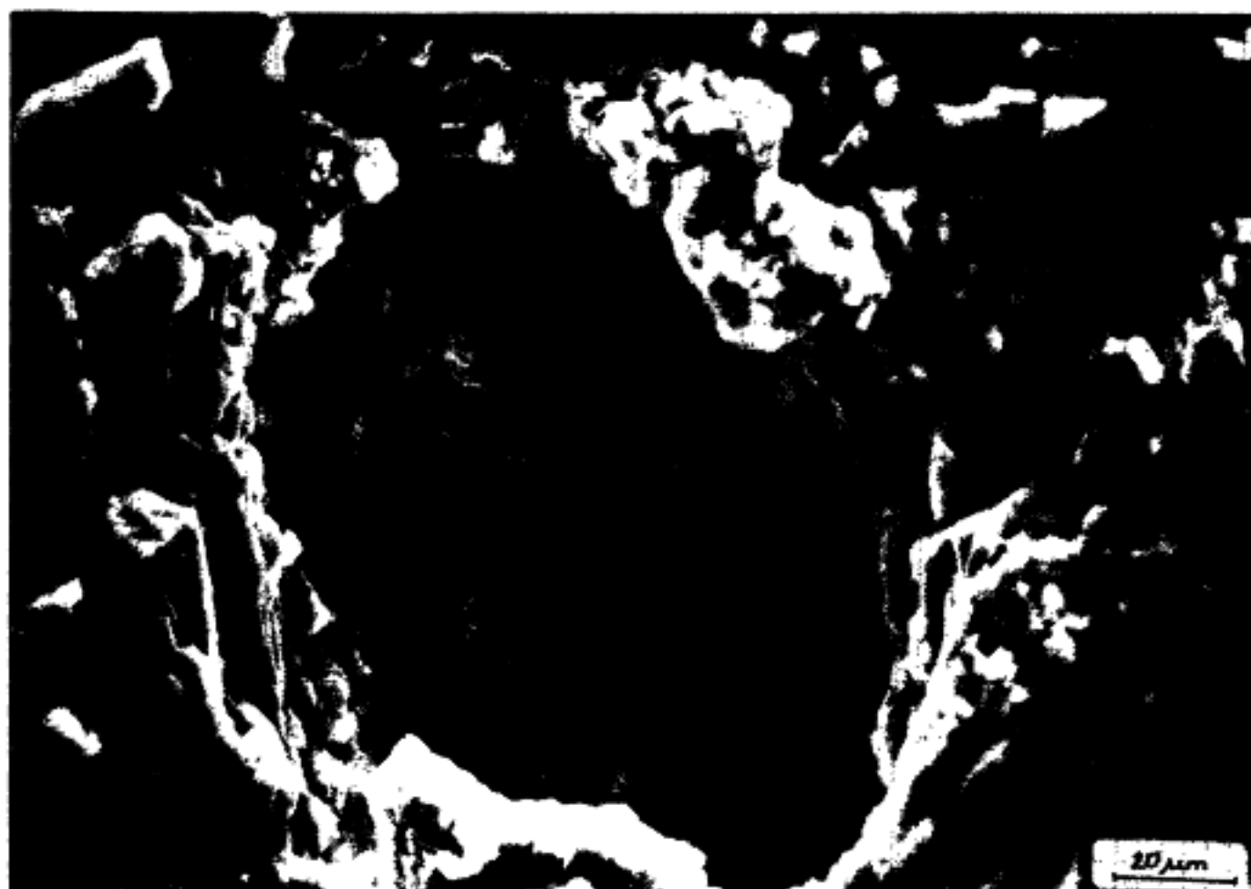
Fig. 7 Vesicle in chondrule from Fig. 5.
