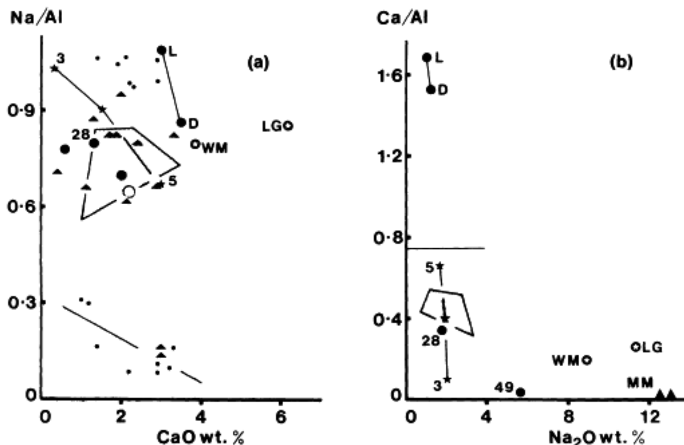
Fig. 4 (a) Na/Al atomic ratio vs. CaO in wt.%. Dots: Manych droplet chondrules; solid circles: Manych glasses (Dodd, 1978b); triangles: Manych microporphyritic chondrules (Dodd, 1978a). Shaded area: Bishunpur dark matrix (this work) includes average opaque matrices of Tieschitz and Bishunpur (Huss et al. , 1981); the open circle on the lower margin is the L-group mean (Dodd, 1978b). Solid stars, (3)–(5): Tieschitz black matrix, Table 1. WM and LG = white matrix and lilac glass (Tieschitz, Table 1). 28 = glass selvage No. 28 from Dodd (1978b). L and D = light and dark glasses (see No. 36 in Dodd, 1978b). The line, lower left, is the best fit to the low Na/Al points. (b) Ca/Al atomic ratio vs. Na 2 O in wt.% shows extremes in Ca/Al ratios in Manych chondrules and glasses (Dodd, 1978a,b) and extreme Na 2 O enrichment coupled with very low Ca/Al in the mesostasis of a Mezö-Madaras chondrule (MM), No. XXI of Kurat (1967). 49 = Manych nepheline normative droplet chondrule (Dodd, 1978b); remaining symbols as in (a). Horizontal line represents the mean ordinary chondritic Ca/Al, 0.74.
