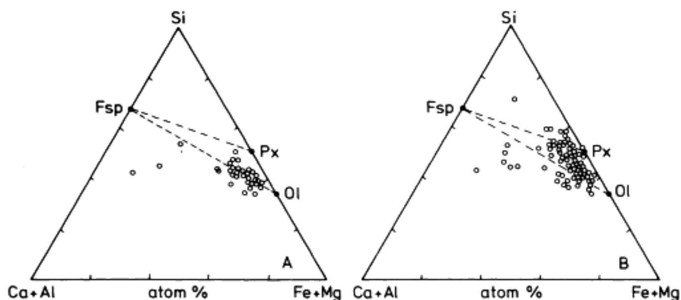
Fig. 3 Composition of chondrules with clear glass (a) and with devitrified glass (b), in atom.%, from Sharps. Symbols as in Fig. 2. Fragments are not shown, because they plot very similar to normal chondrules.
