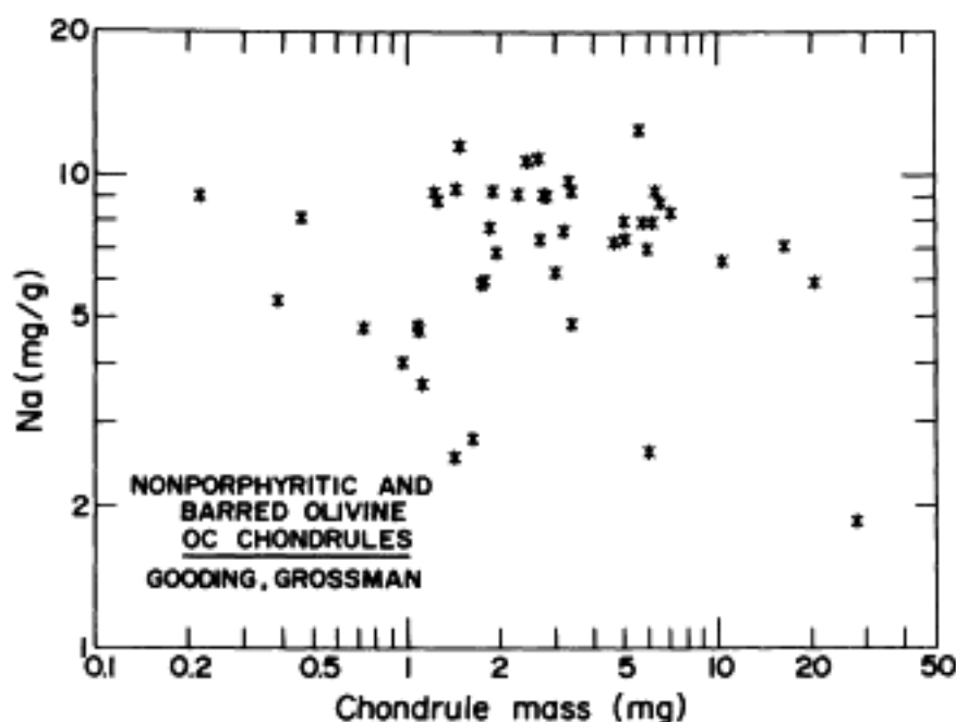
Fig. 8 Sodium concentration vs. chondrule mass for only those chondrules that clearly were fully molten droplets. The non-porphyrific chondrules from Gooding (1979) and from Grossman and Wasson (1982, 1983) are shown. Even for this subset, no correlation of volatile content with mass is observed.
