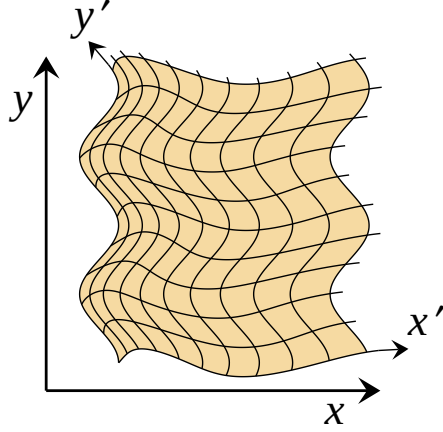
Figure 1: A transition from one coordinate frame \{x, y\} to an other, curved coordinate frame \{x', y'\} .
