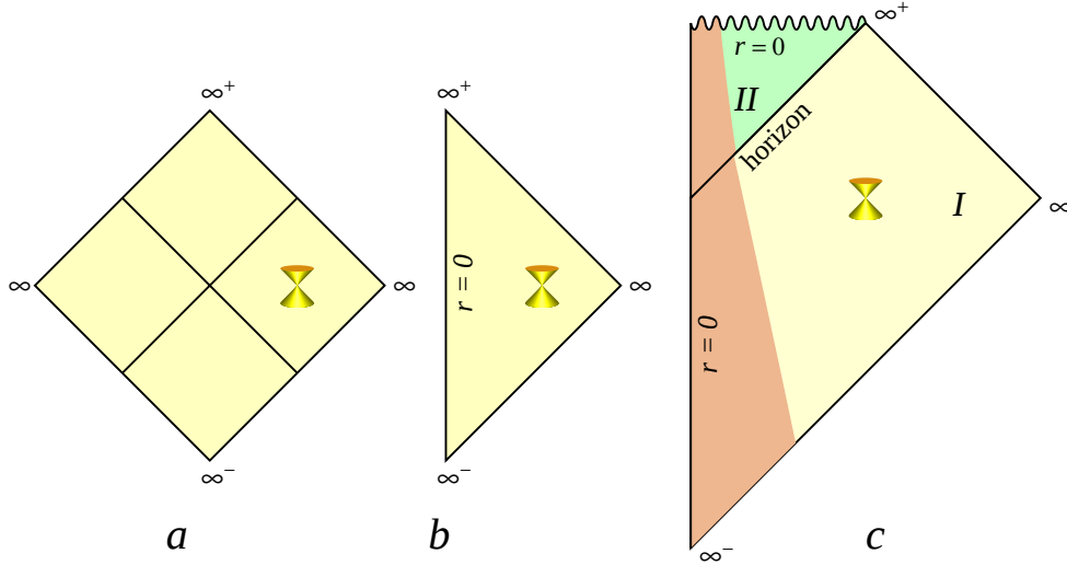
Figure 5: a ) Penrose diagram for the Minkowski vacuum with Cartesian transverse coordinates, b ) Minkowski space in polar coordinates; c ) Penrose diagram for a black hole formed by matter (darker color represents matter falling in).
