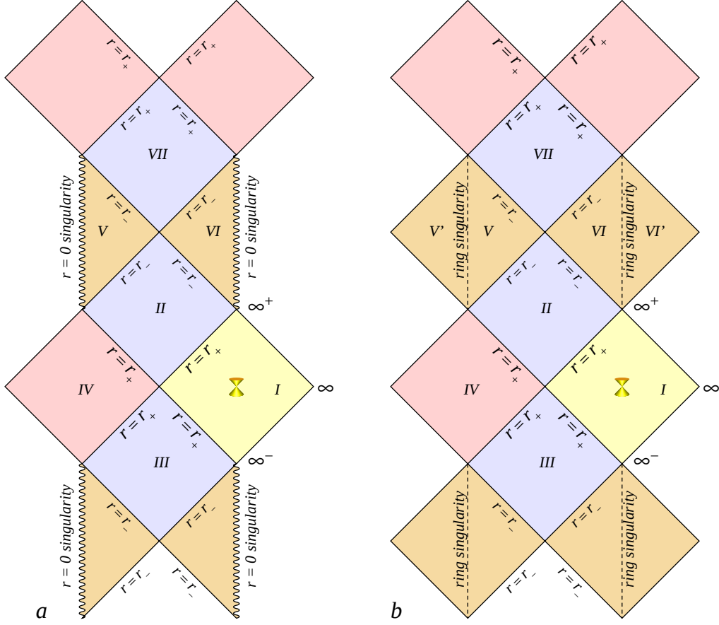
Figure 6: Penrose diagram for the Reissner-Nordström (a) and the Kerr black hole (b). The singularity at r = 0 is a natural boundary in case of Reissner-Nordström, but it is a ring singularity in case of Kerr- and Kerr-Newman, through which one can continue to asymptotically flat universes V' and VI' , containing a negative mass Kerr Newman black hole.
