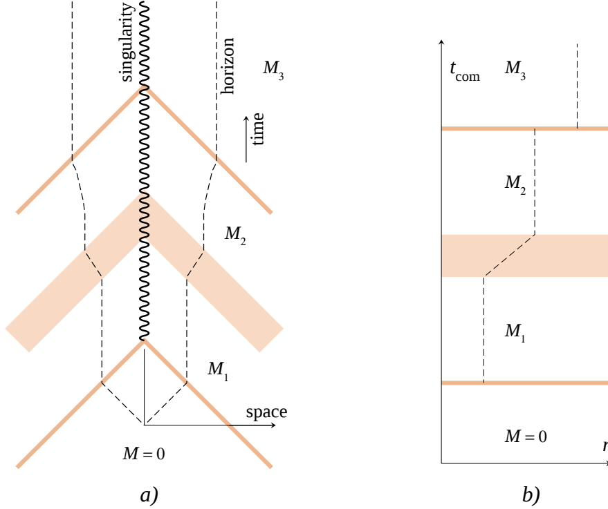
Figure 3: Several shells of matter (shaded lines) implode to form a black hole, whose mass M increases. In a ), time is neither the Schwarzschild time nor the t_{\text{com}} coordinate, but it indicates the causal order of events. The dotted line is the location of the horizon. In b ), the coordinates t_{\text{com}} and r are used. The dotted line here is the apparent Schwarzschild horizon r = 2M . Here, 0 < M_1 < M_2 < M_3 .
