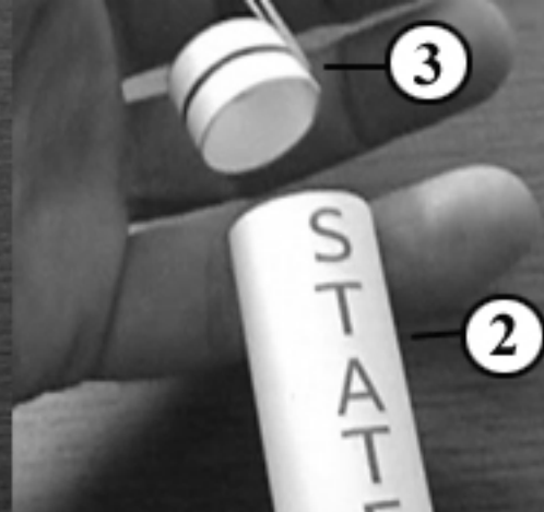
Test fit of adaptor ring #3 and glue into top of #2
